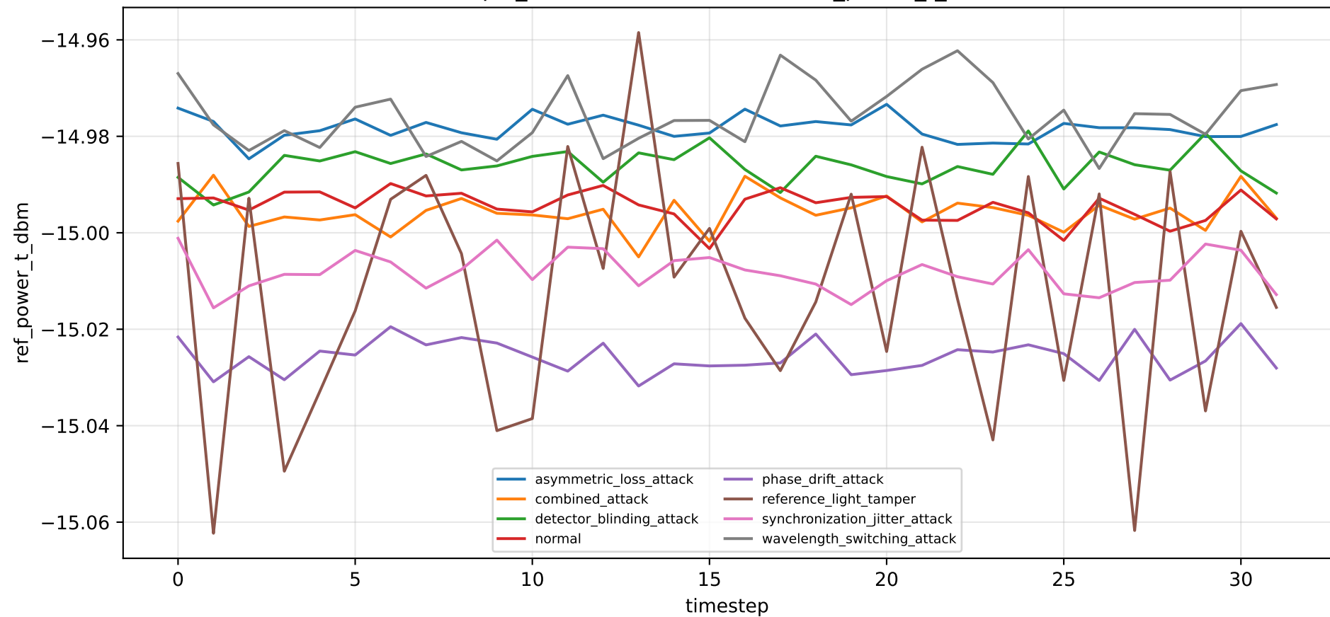
tfqkd_clean: drift over time — ref_power_t_dbm
