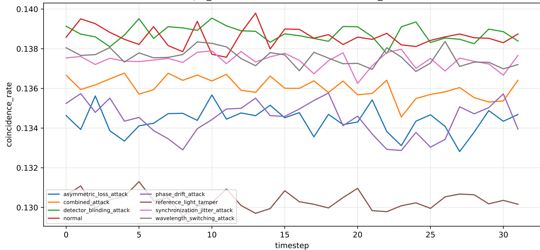
tfqkd_clean: drift over time — coincidence_rate
