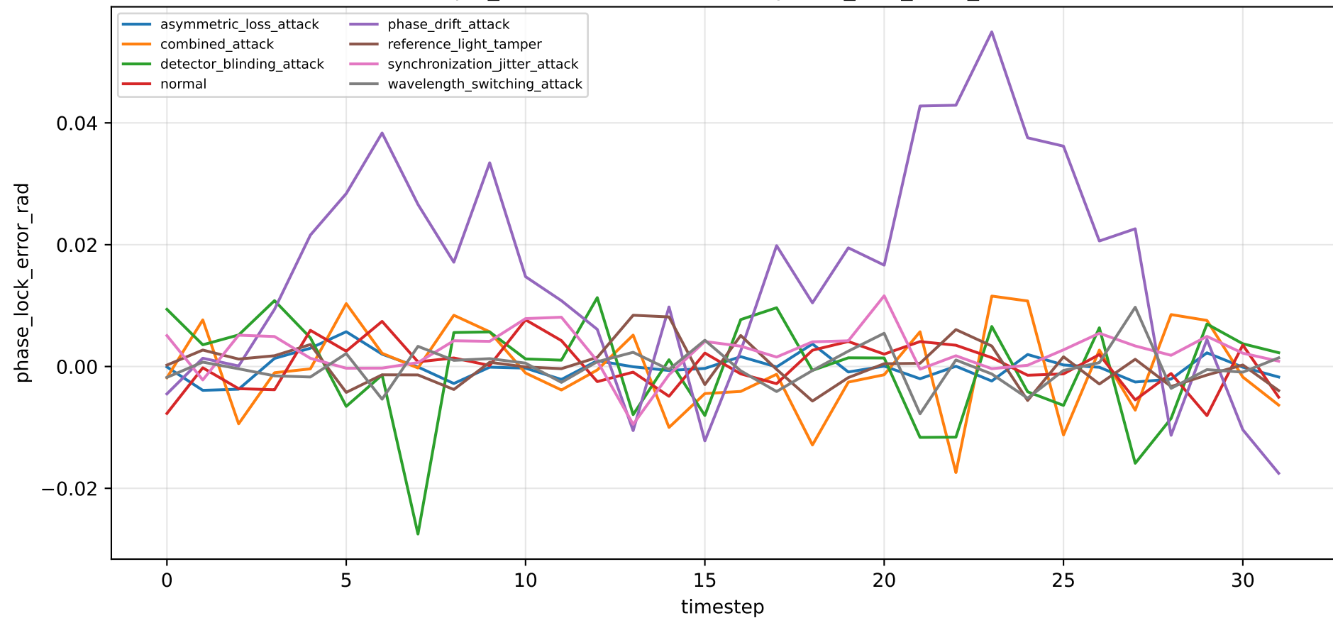
tfqkd_clean: drift over time — phase_lock_error_rad
