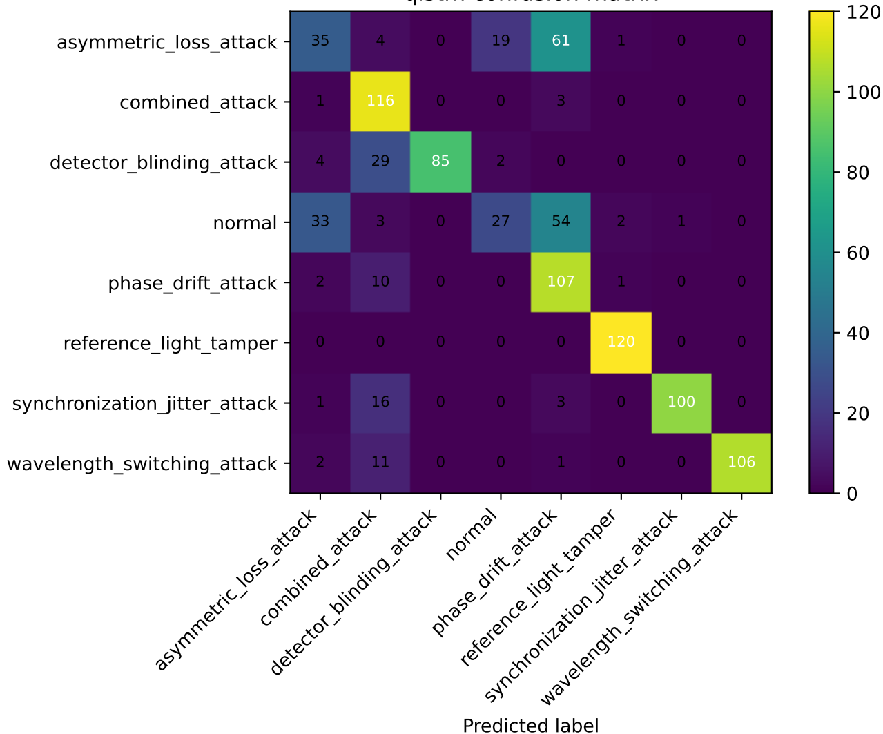
qlstm confusion matrix
