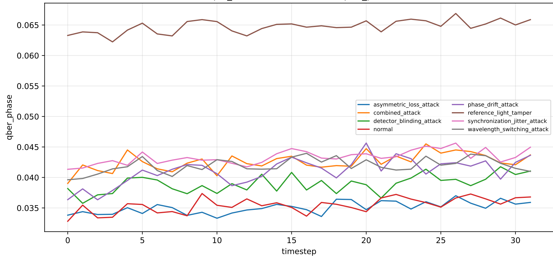
tfqkd_drift: drift over time — qber_phase
