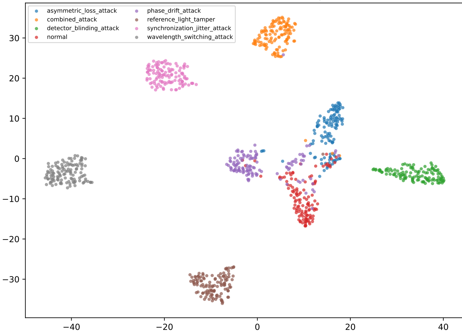
t-SNE of transformer embeddings
