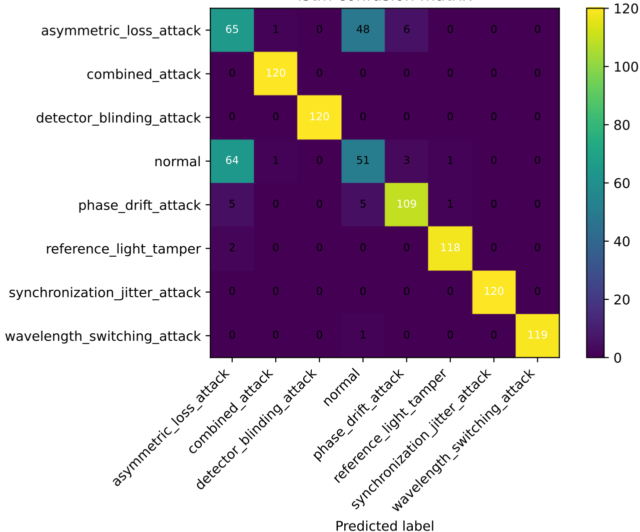
Istm confusion matrix
