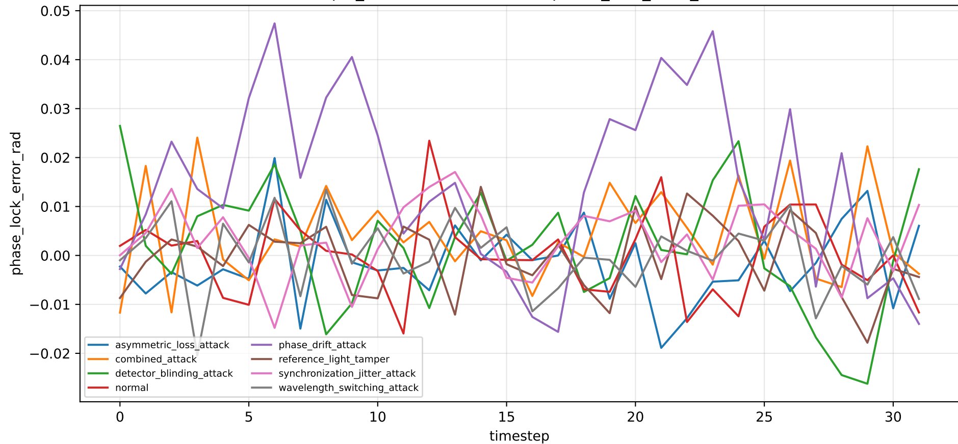
tfqkd_drift: drift over time — phase_lock_error_rad
