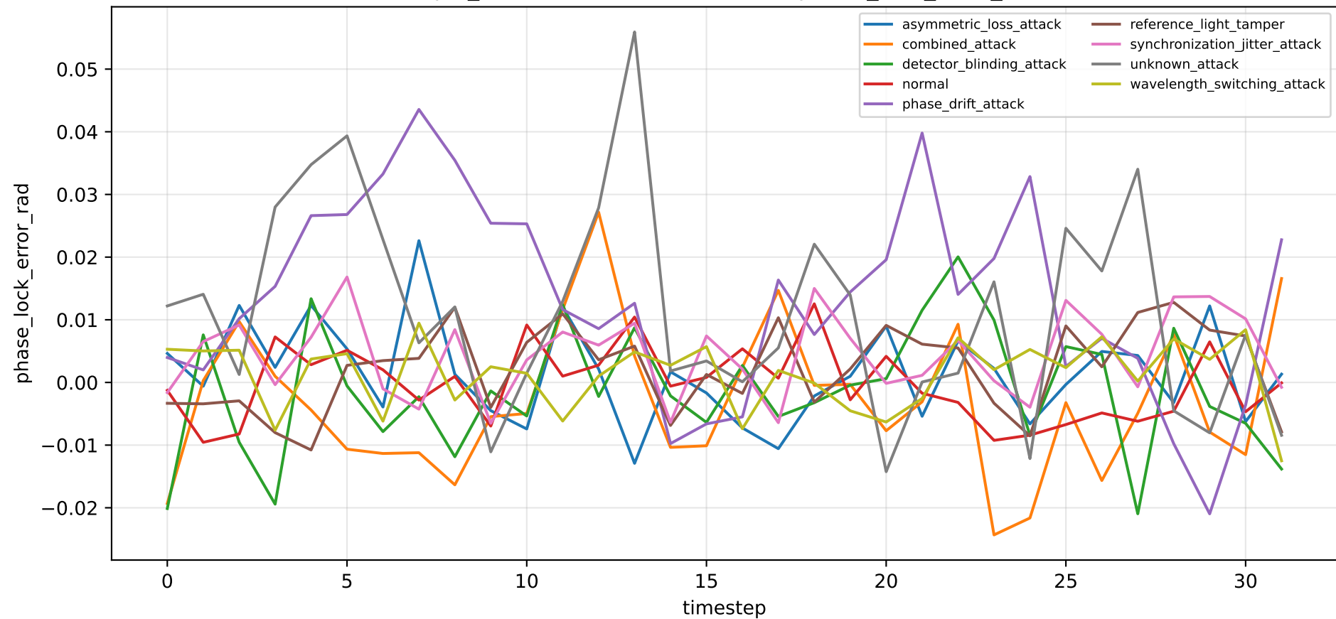
tfqkd_unknown: drift over time — phase_lock_error_rad
