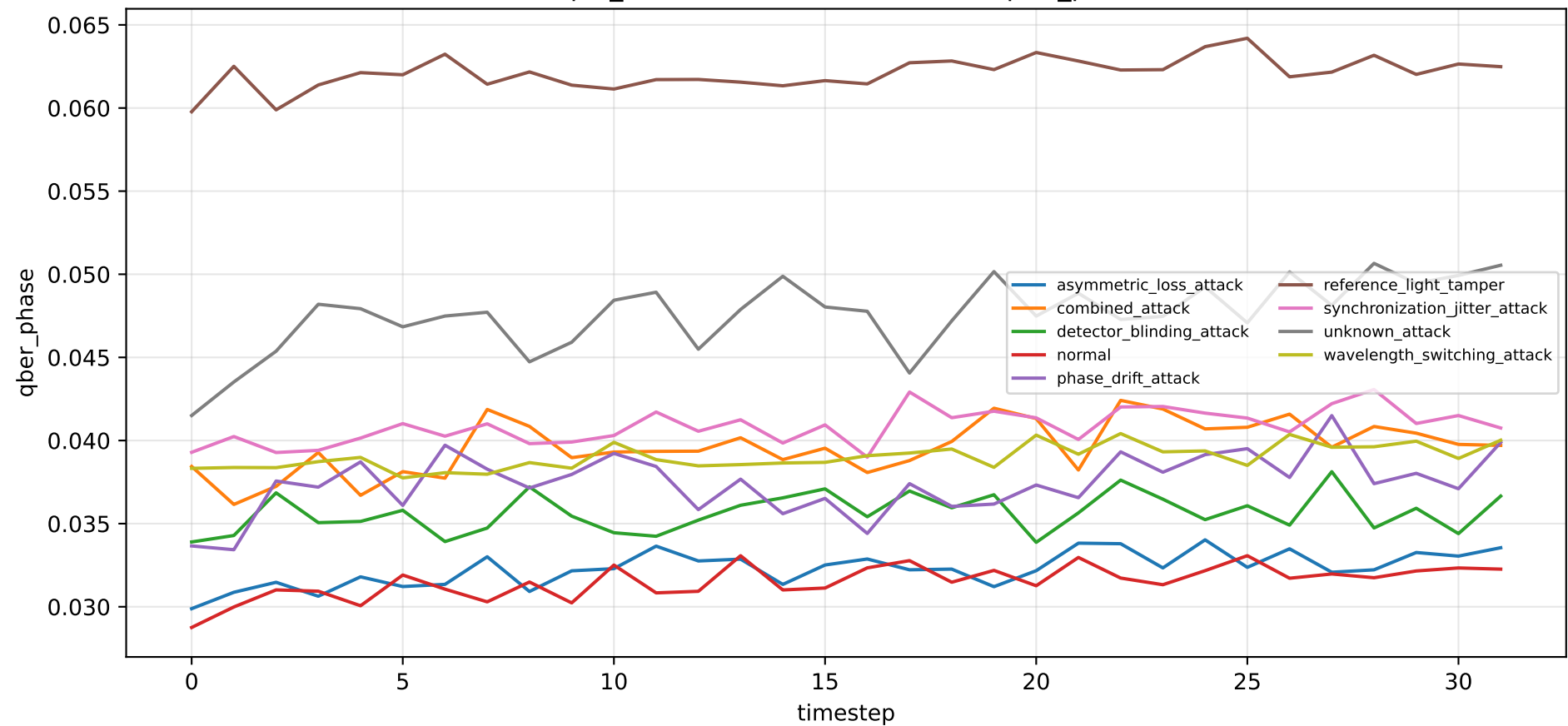
tfqkd_unknown: drift over time — qber_phase
