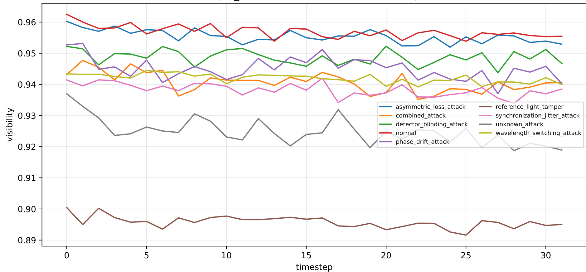
tfqkd_unknown: drift over time — visibility
