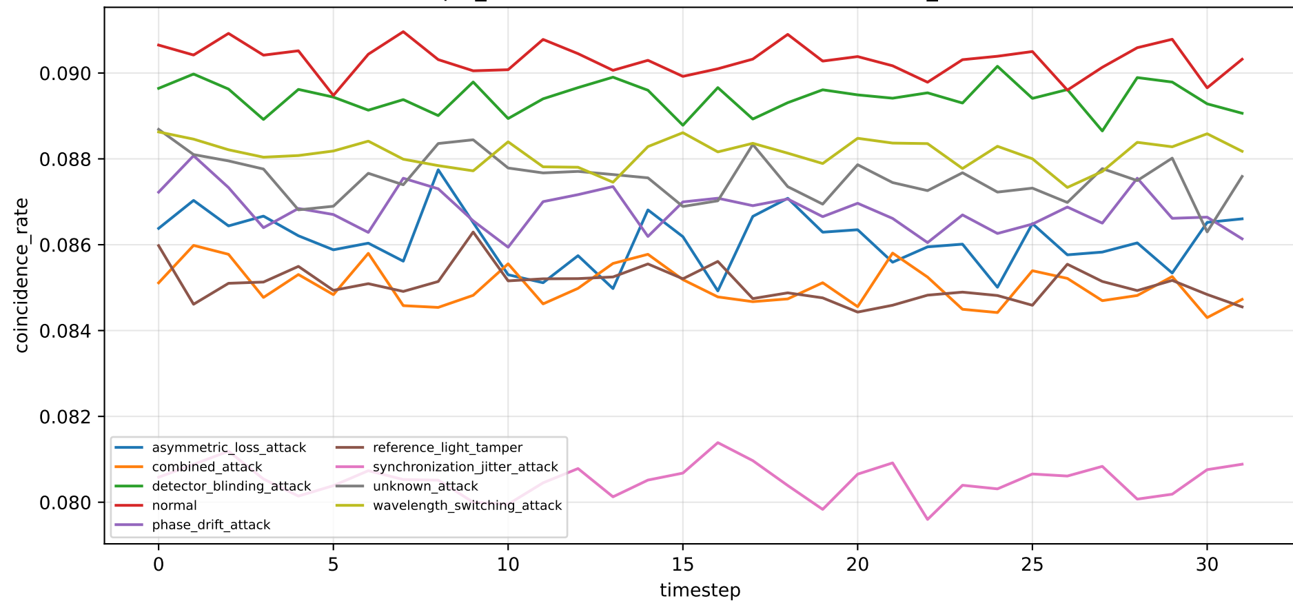
tfqkd_unknown: drift over time — coincidence_rate
