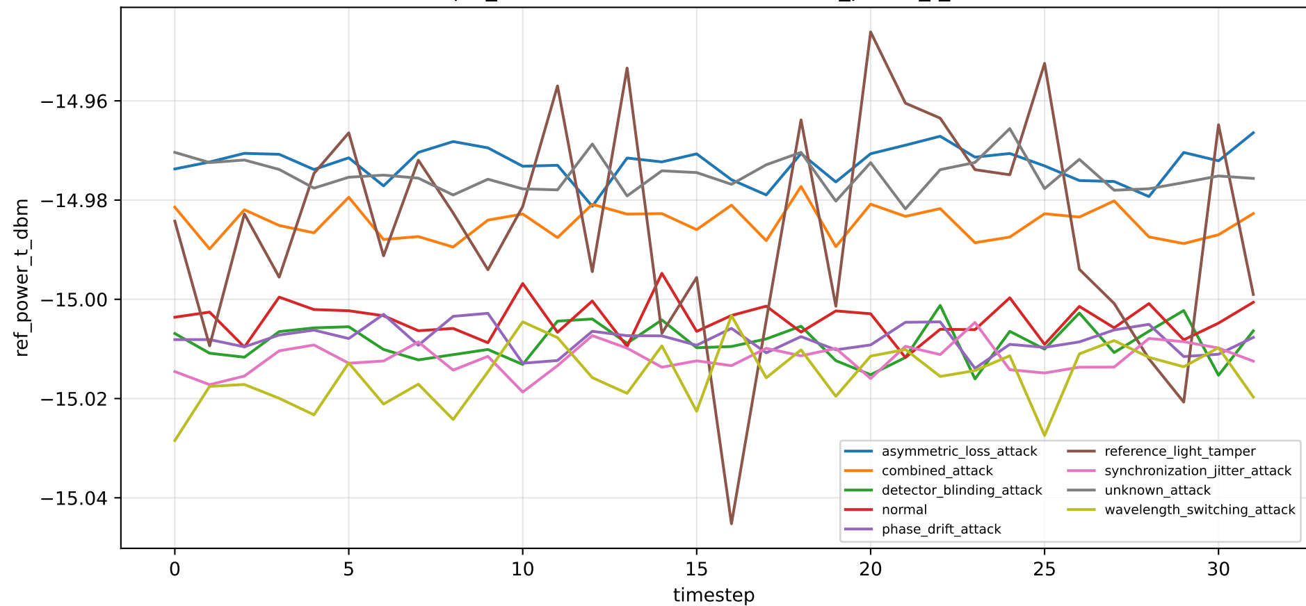
tfqkd_unknown: drift over time — ref_power_t_dbm
