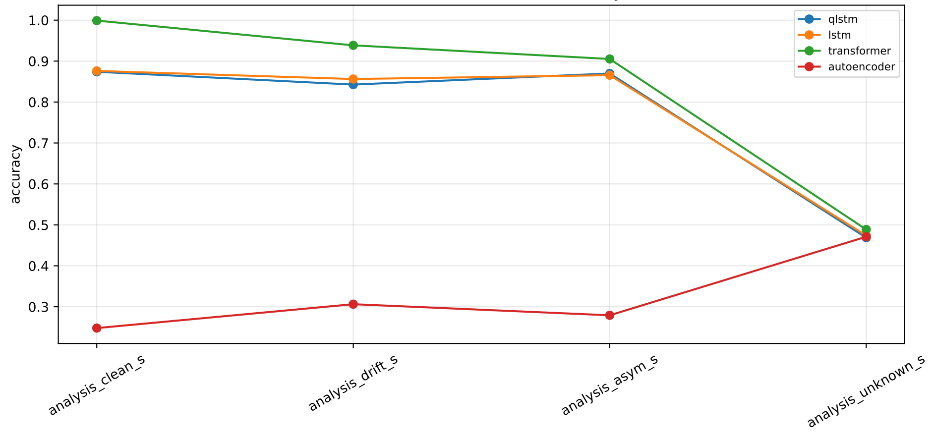
Cross-domain robustness: accuracy
