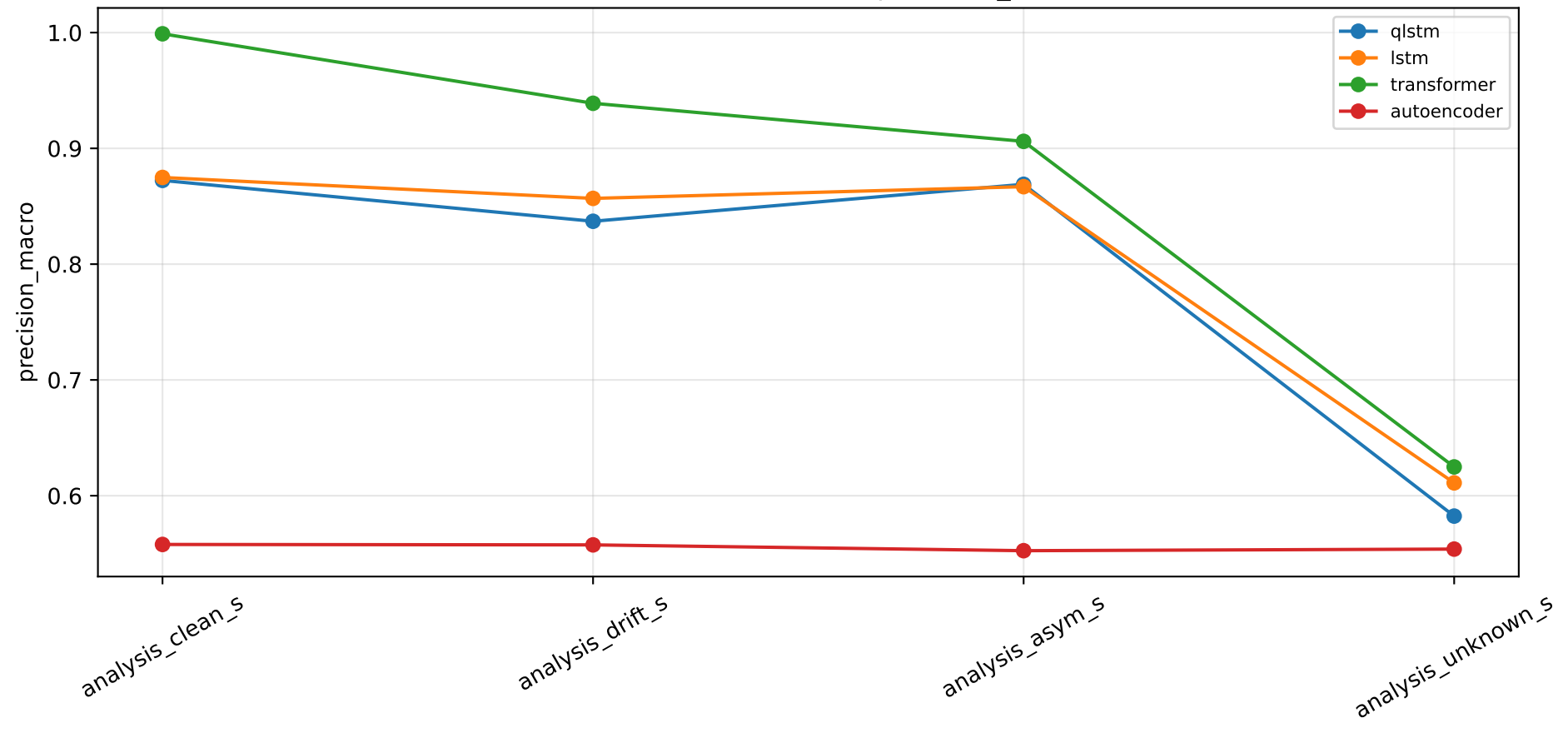
Cross-domain robustness: precision_macro
