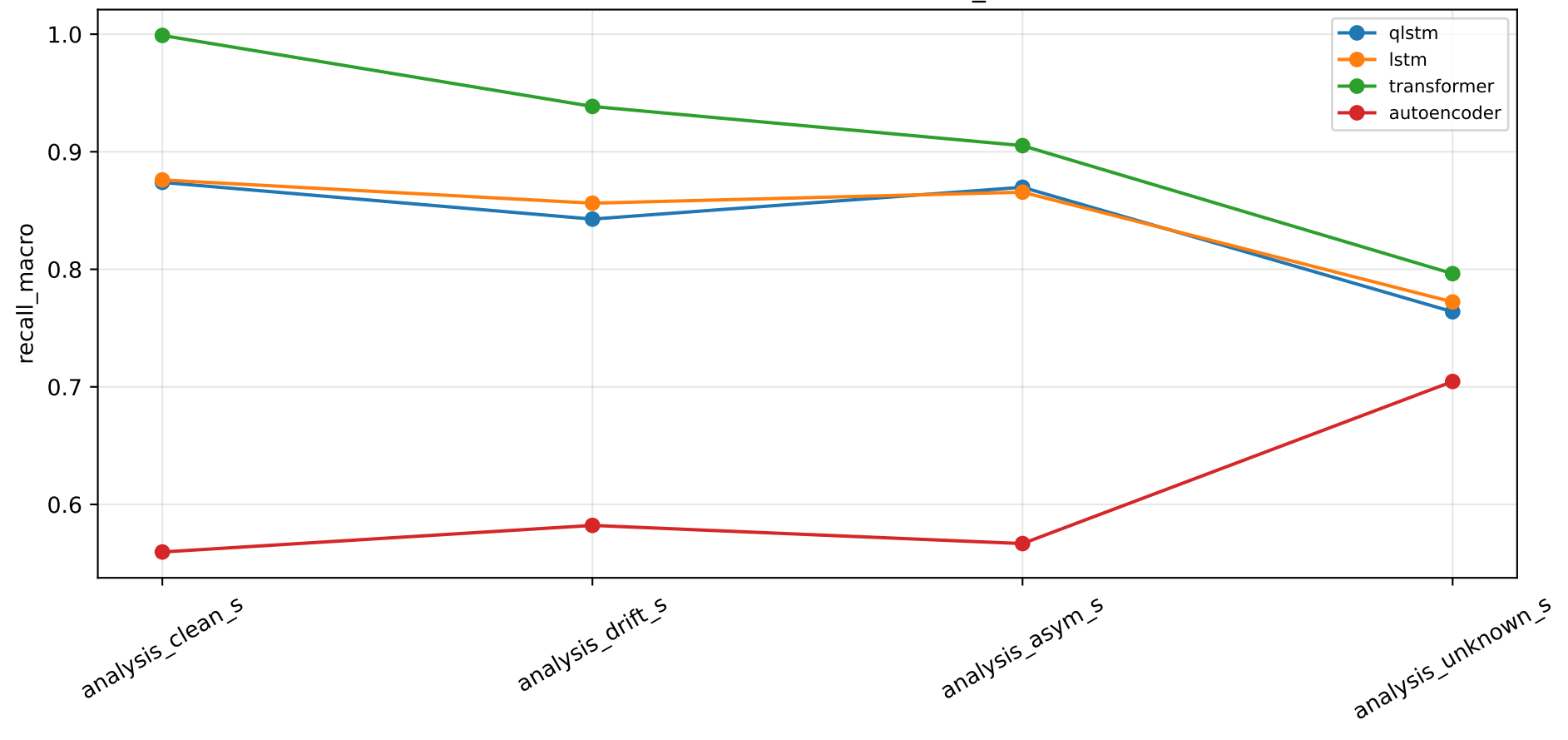
Cross-domain robustness: recall_macro
