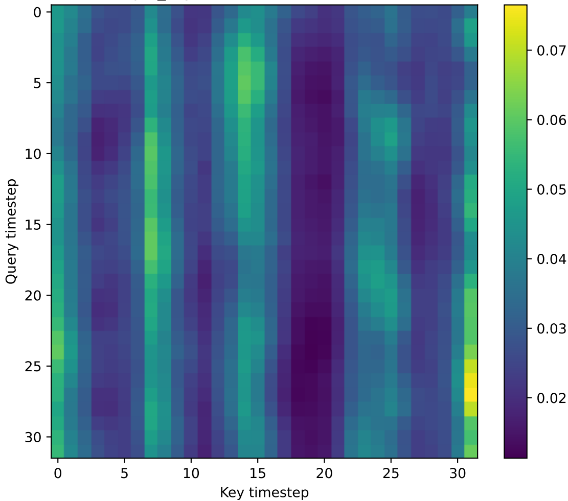
tfqkd_asym — transformer attention
