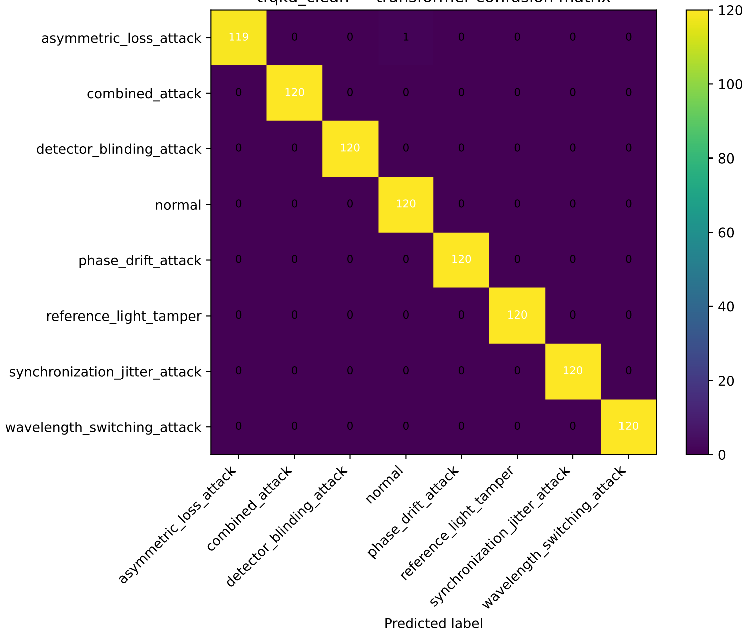
tfqkd_clean — transformer confusion matrix
