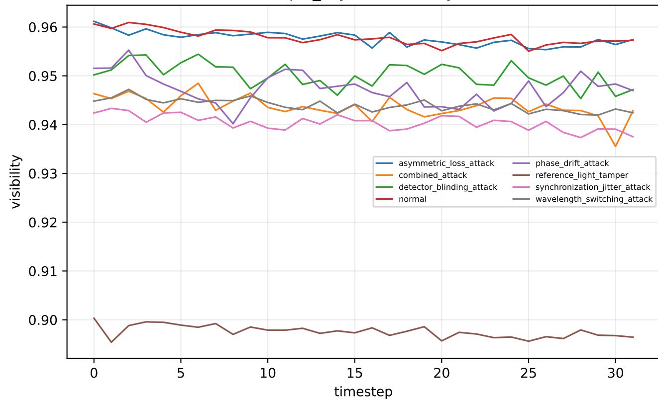
tfqkd_asym — visibility
