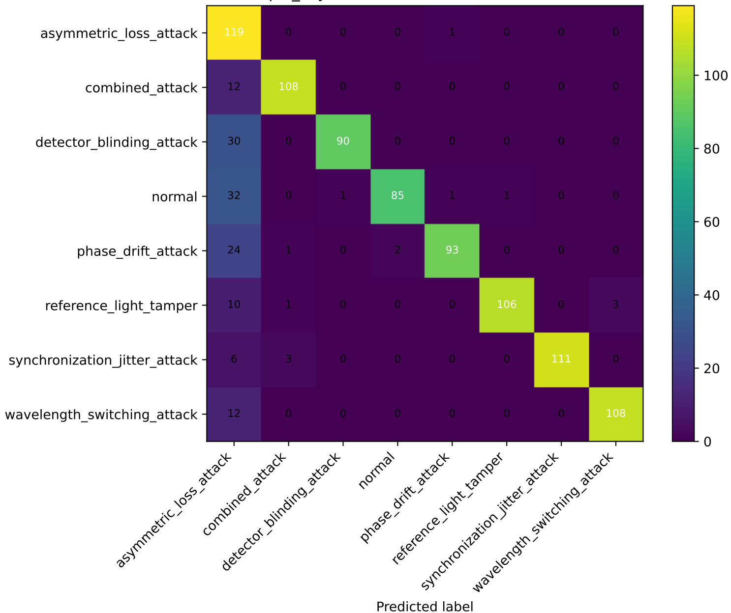
tfqkd_asym — transformer confusion matrix
