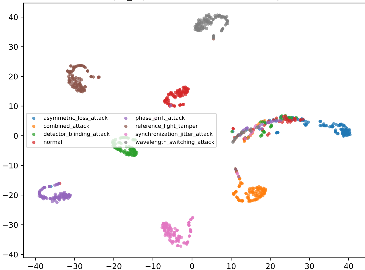
tfqkd_asym — transformer embeddings
