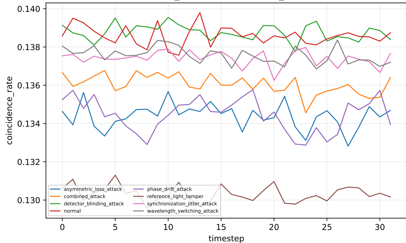
tfqkd_clean — coincidence_rate
