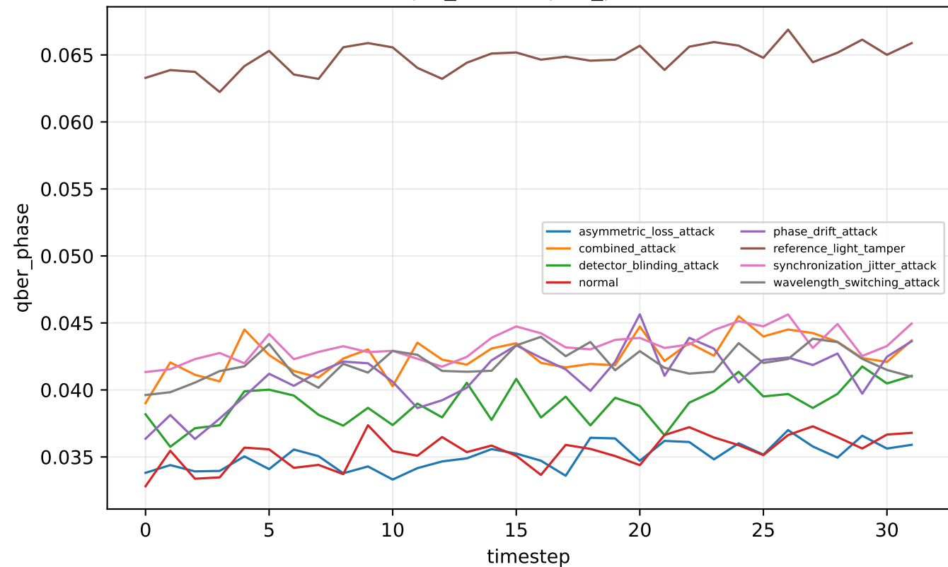
tfqkd_drift — qber_phase
