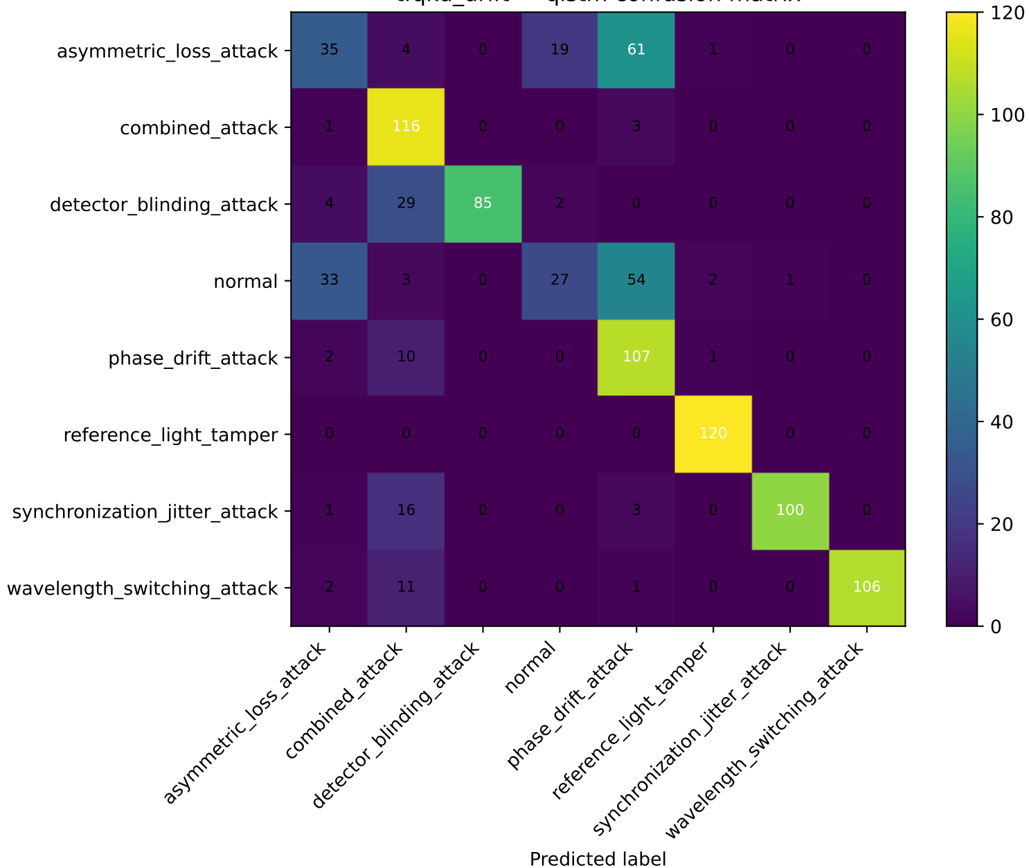
tfqkd_drift — qlstm confusion matrix
