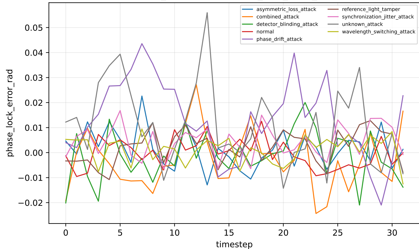
tfqkd_unknown — phase_lock_error_rad
