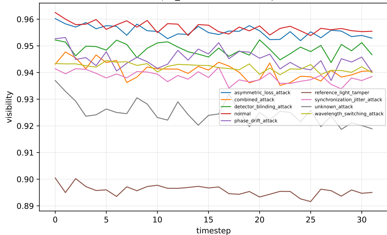
tfqkd_unknown — visibility
