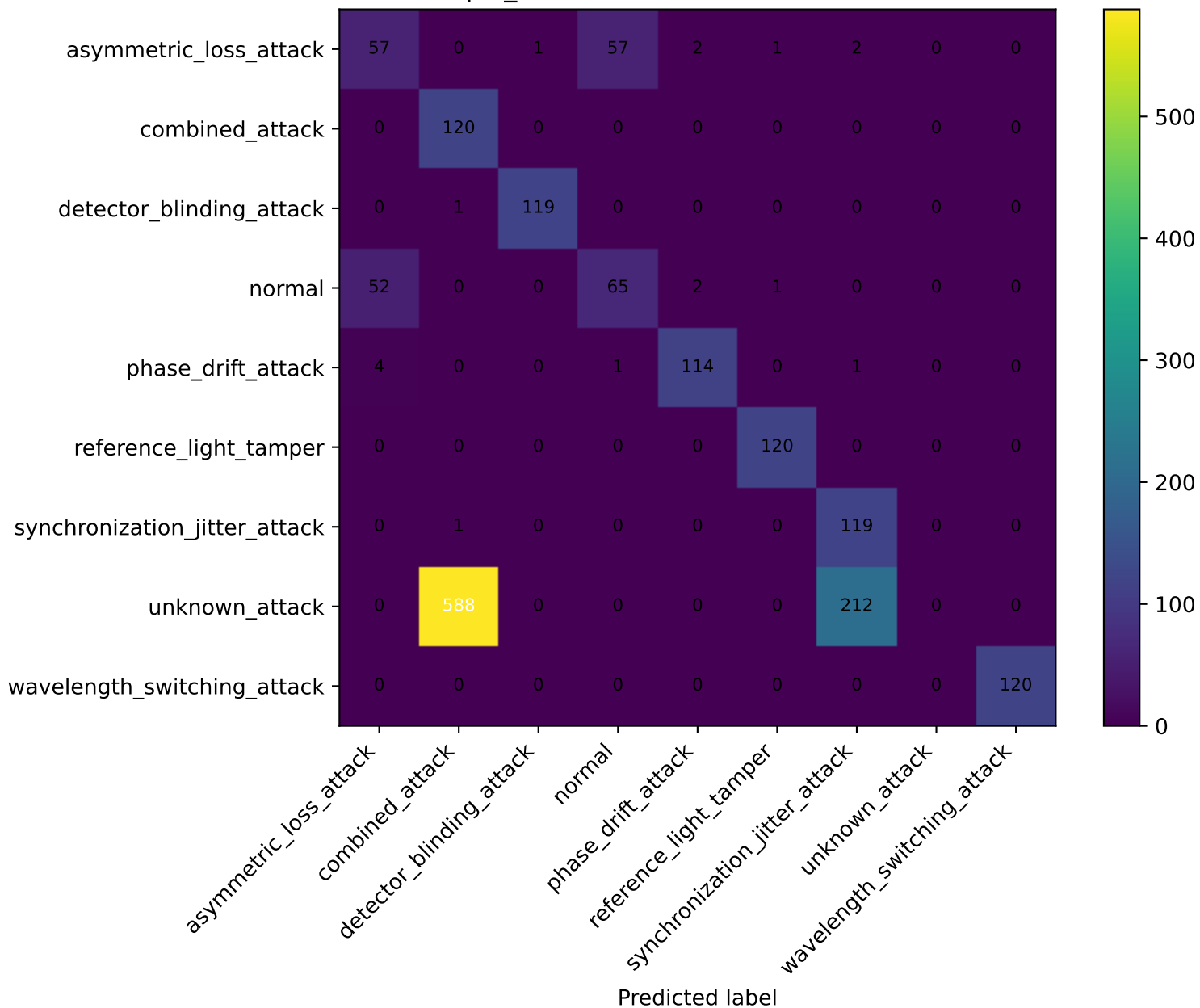
tfqkd_unknown — lstm confusion matrix
