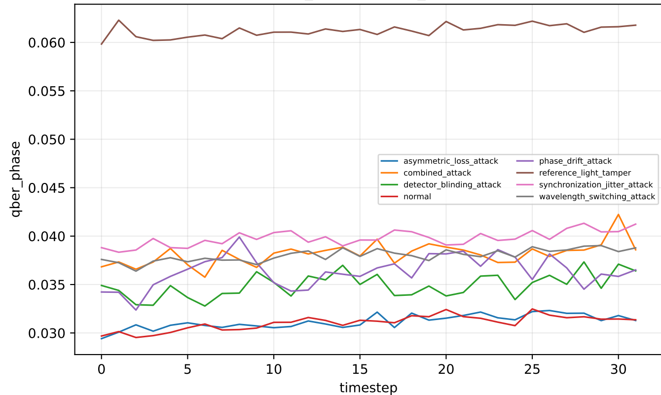
tfqkd_asym — qber_phase
