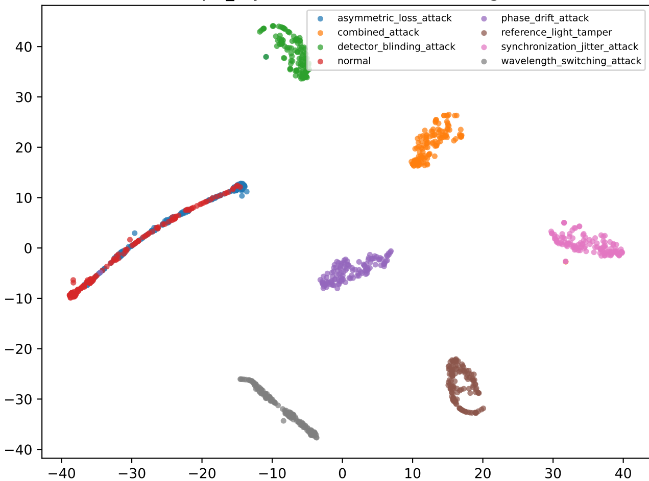
tfqkd_asym — transformer embeddings
