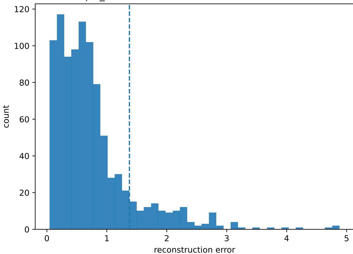
tfqkd_clean — autoencoder reconstruction errors
