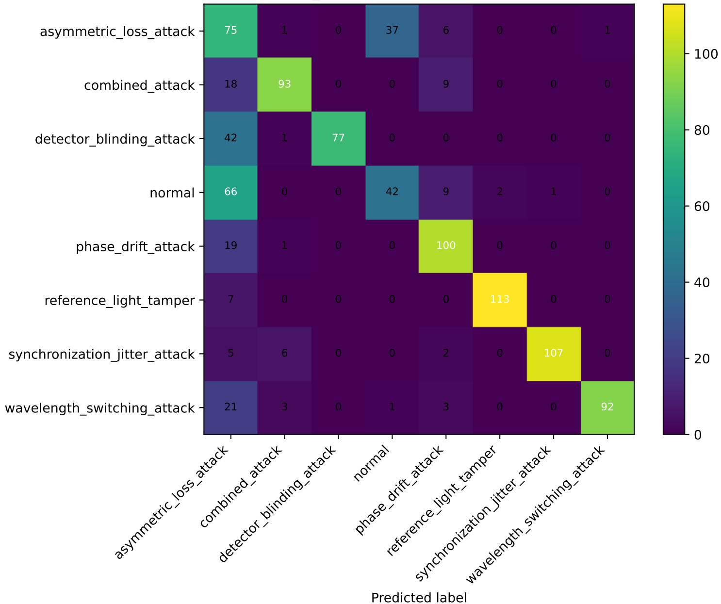
tfqkd_asym — qlstm confusion matrix
