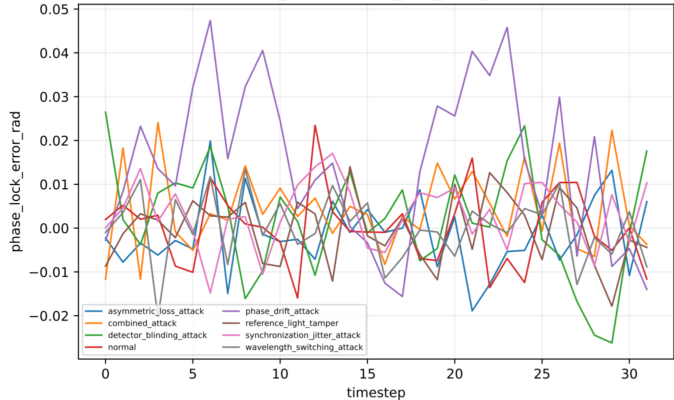
tfqkd_drift — phase_lock_error_rad
