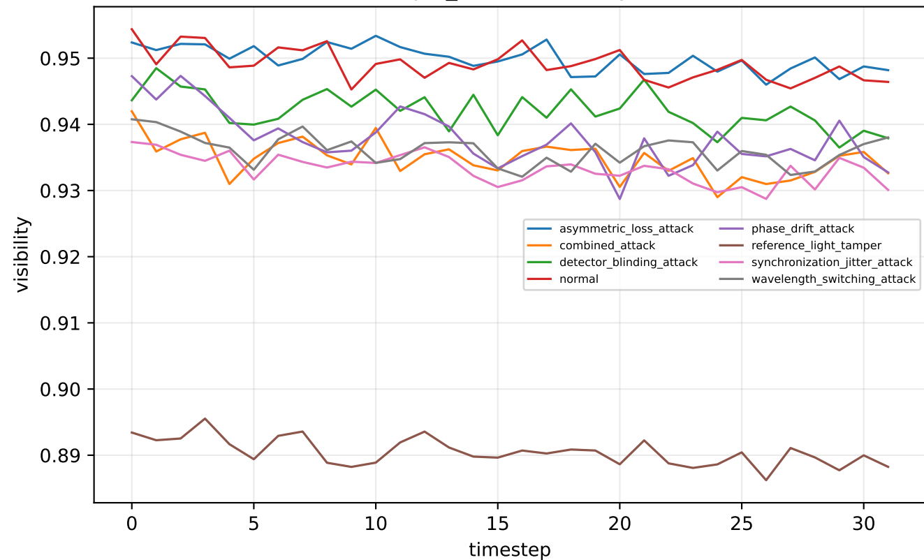
tfqkd_drift — visibility
