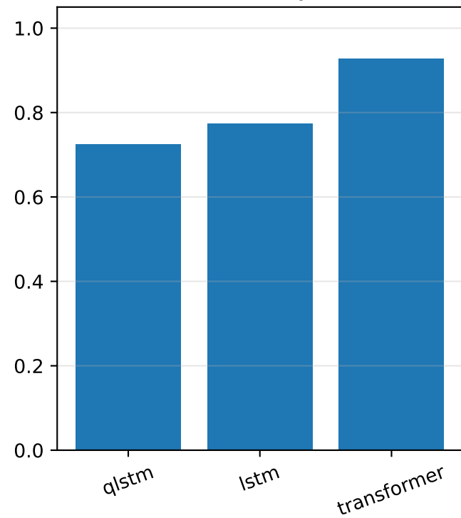
accuracy
