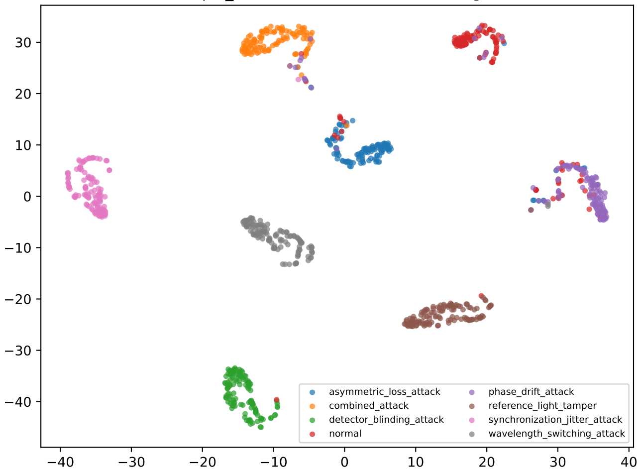
tfqkd_drift — transformer embeddings
