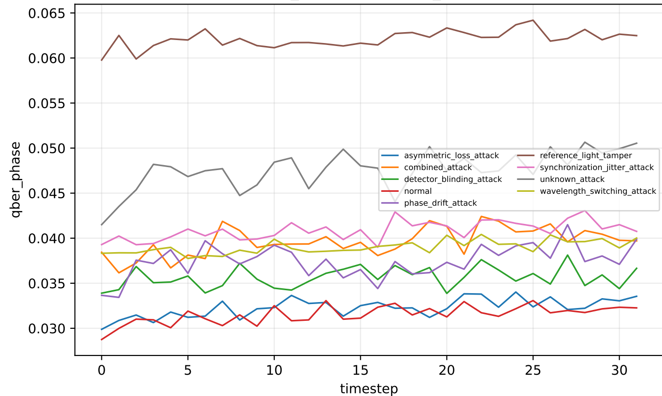
tfqkd_unknown — qber_phase
