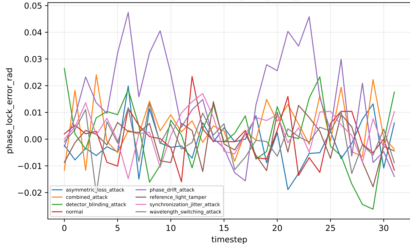
tfqkd_drift — phase_lock_error_rad
