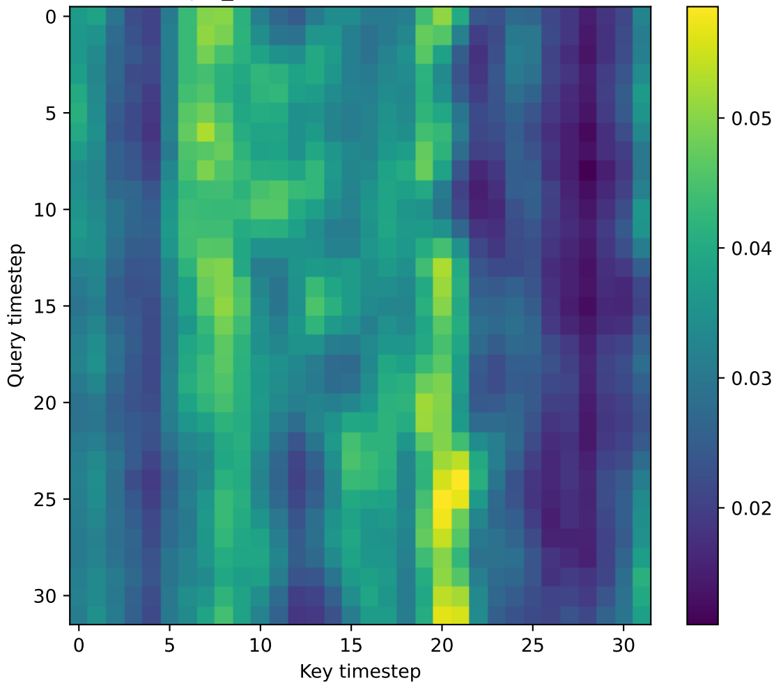
tfqkd_drift — transformer attention
