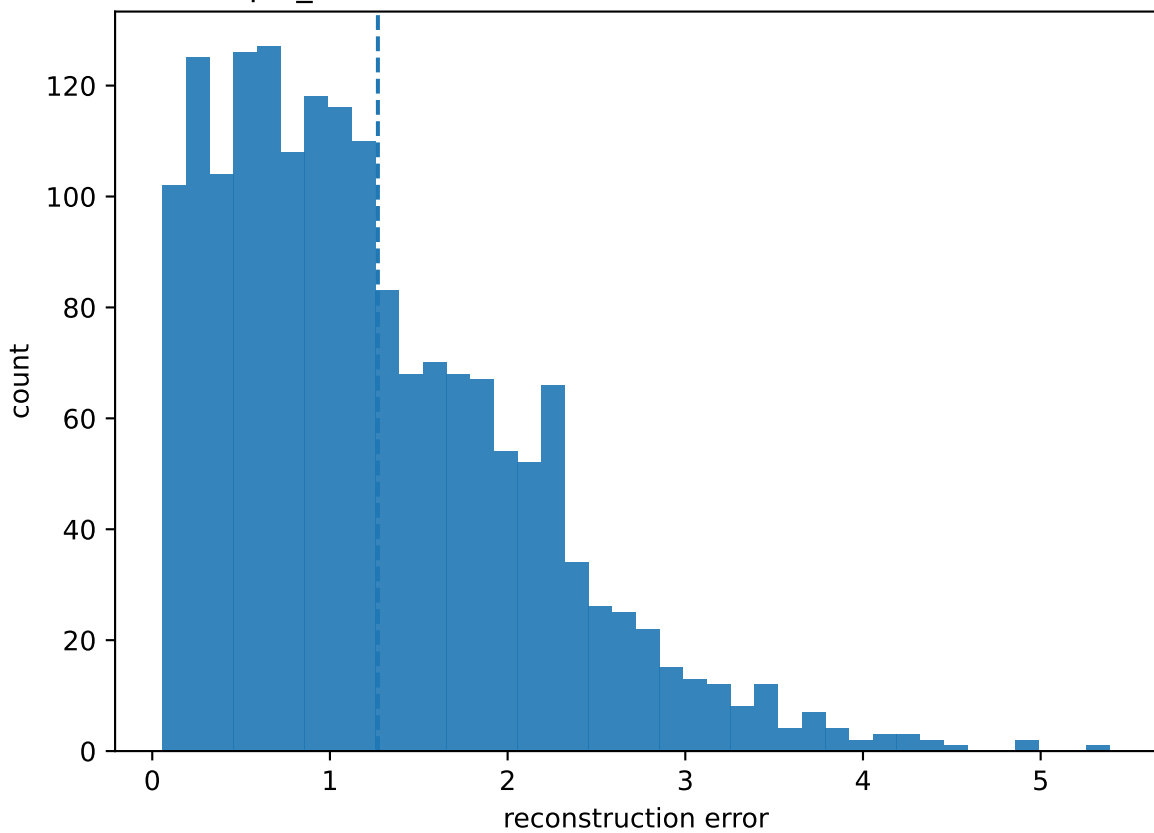
tfqkd_unknown — autoencoder reconstruction errors
