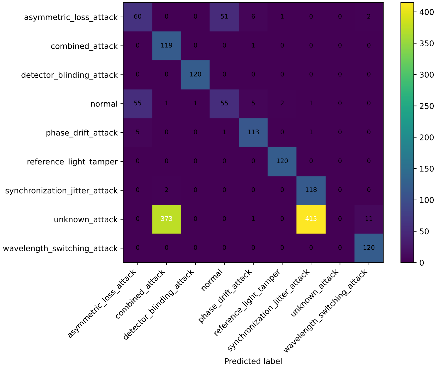
tfqkd_unknown — qlstm confusion matrix
