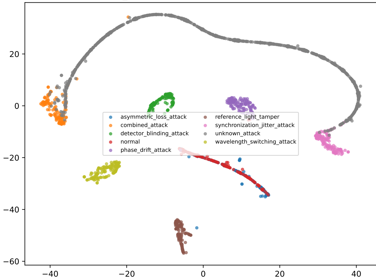
tfqkd_unknown — transformer embeddings
