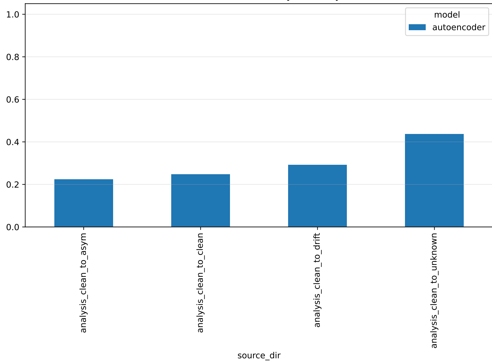
Cross-domain anomaly accuracy
