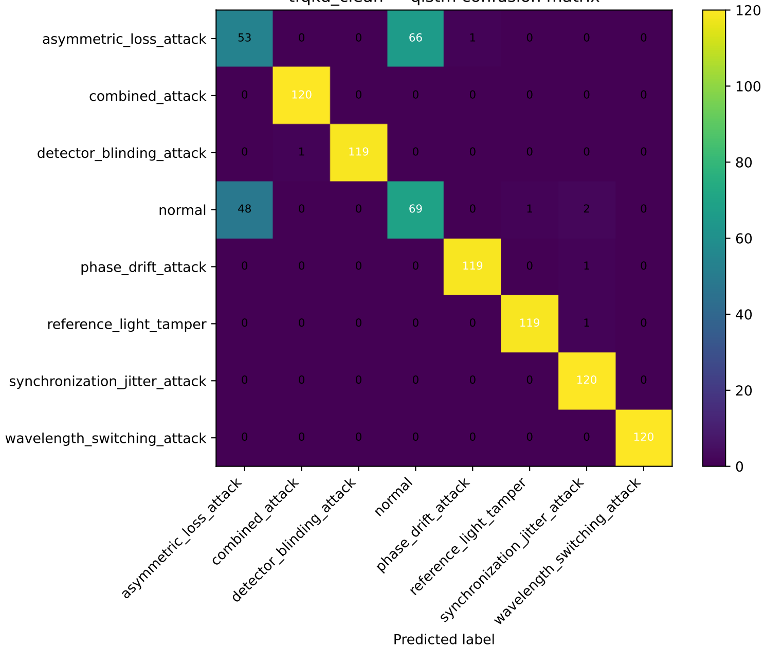
tfqkd_clean — qlstm confusion matrix
