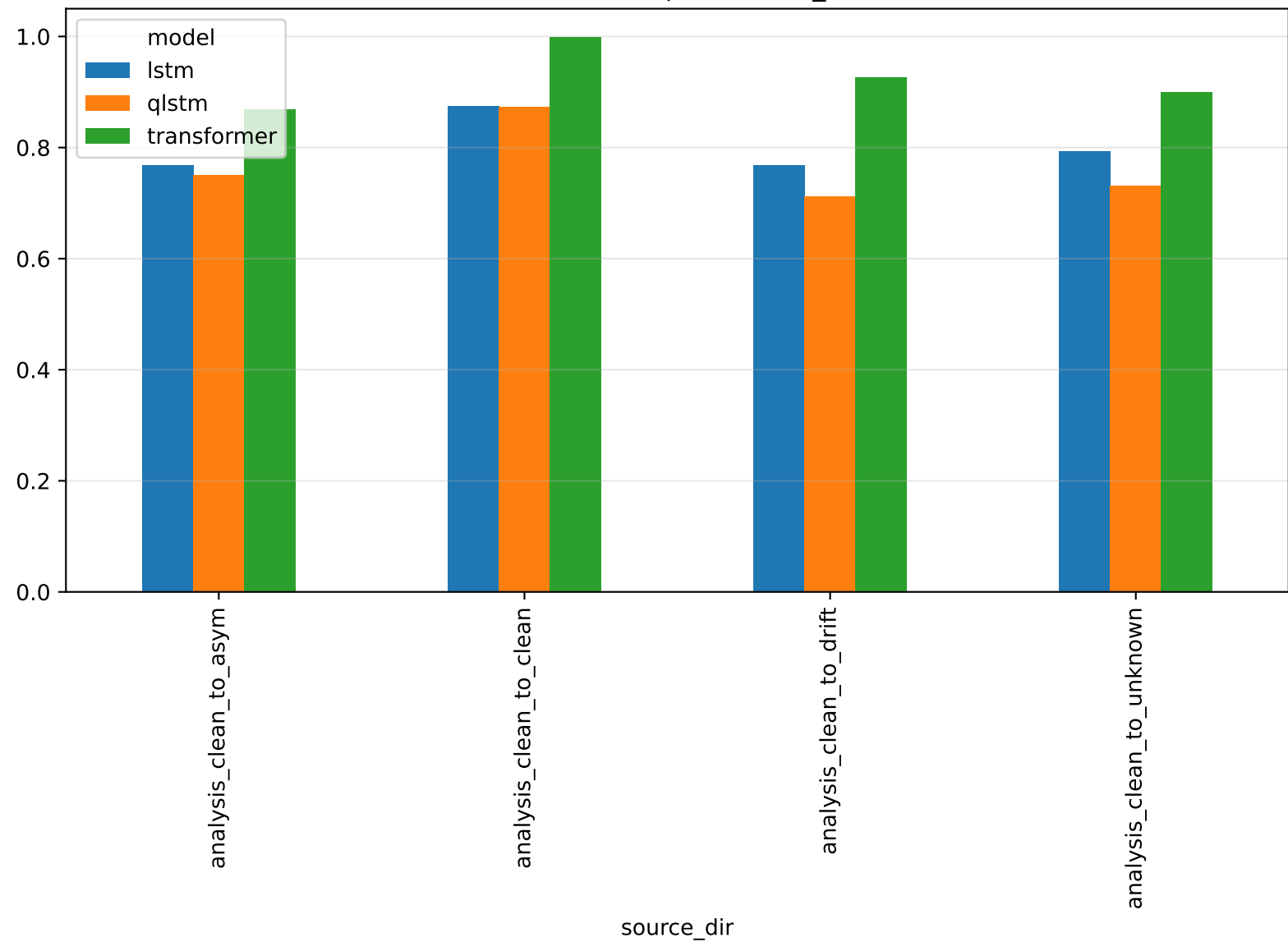
Cross-domain supervised f1_macro
