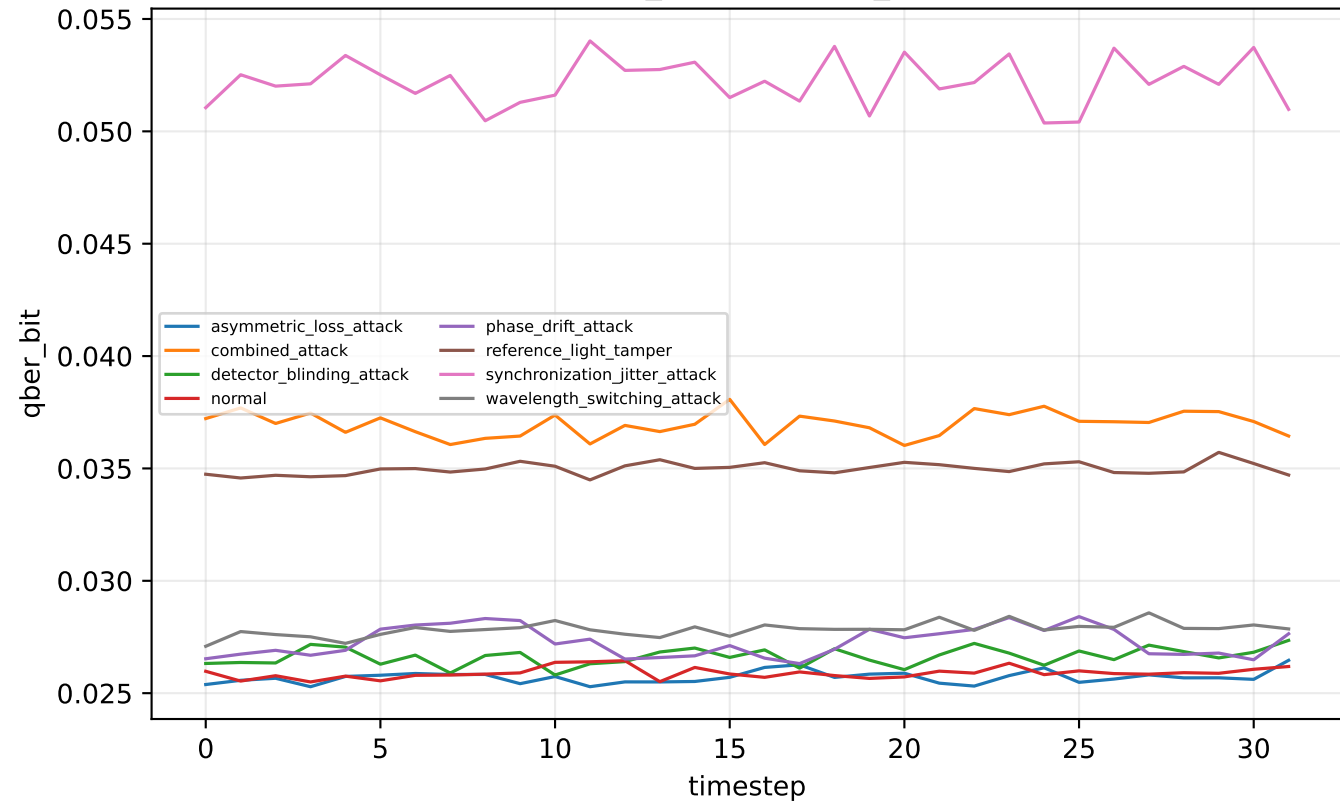
tfqkd_clean — qber_bit
