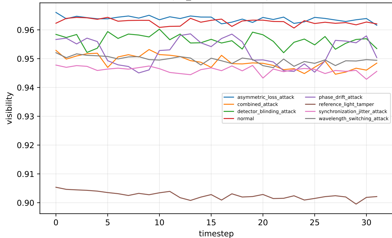
tfqkd_clean — visibility
