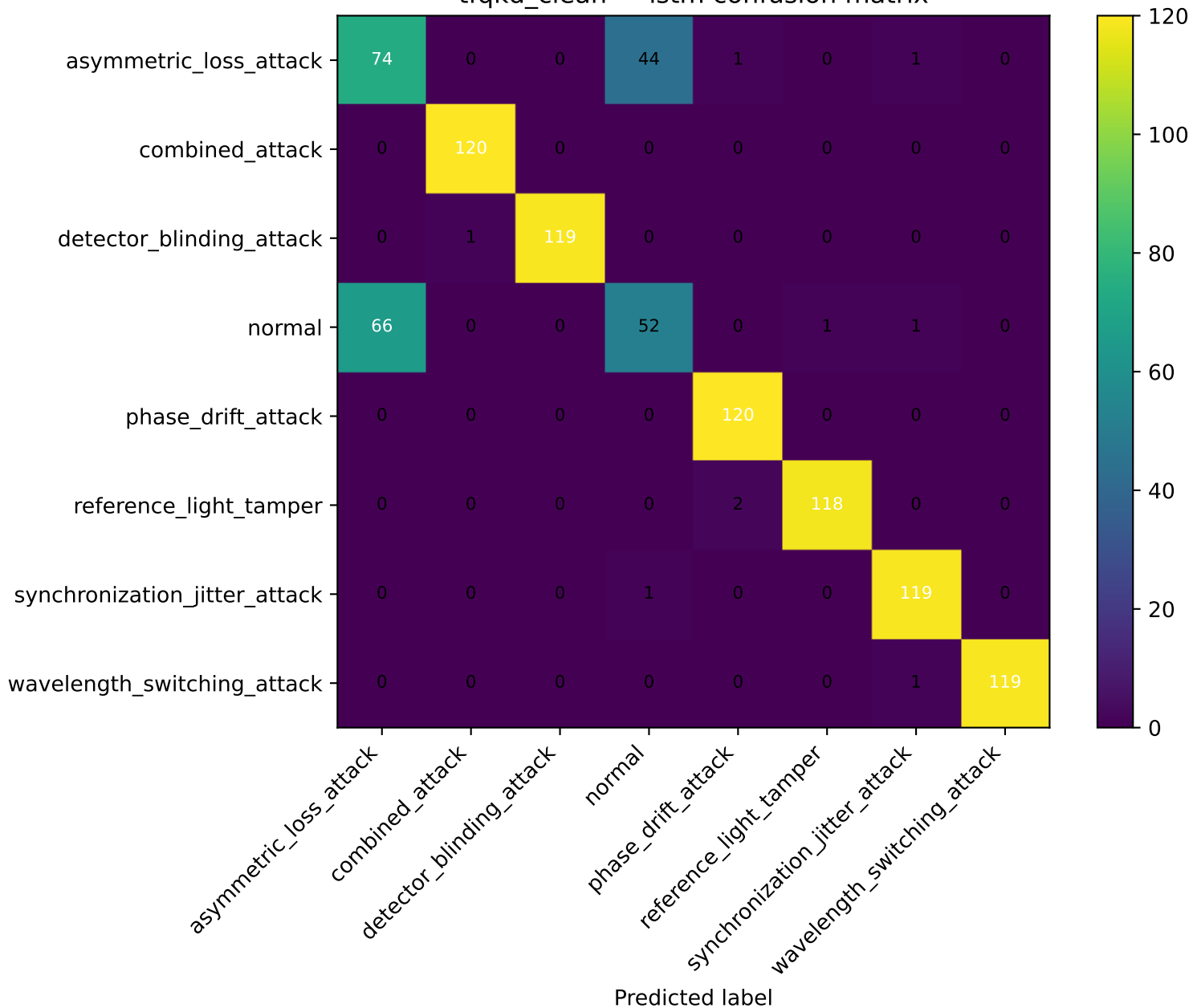
tfqkd_clean — lstm confusion matrix
