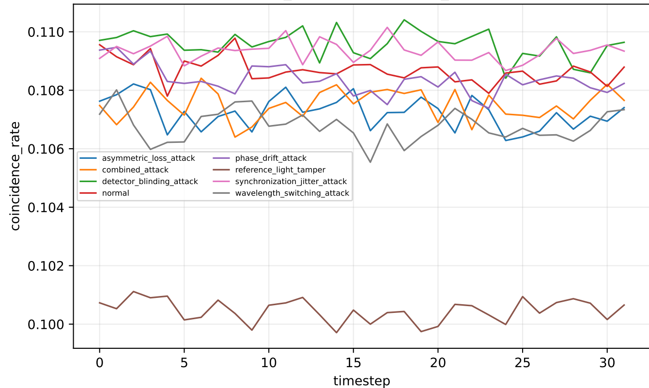
tfqkd_drift — coincidence_rate
