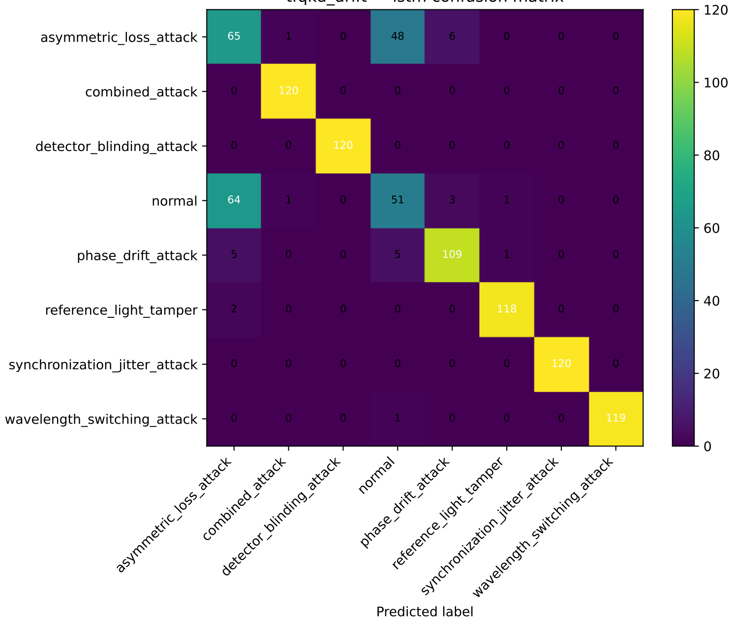
tfqkd_drift — lstm confusion matrix
