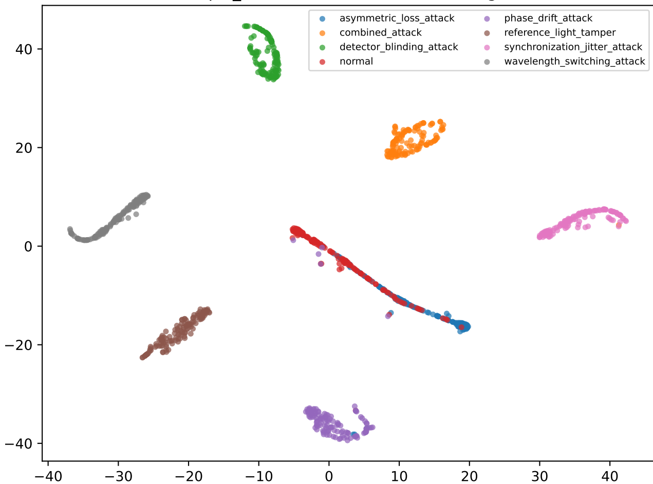
tfqkd_drift — transformer embeddings
